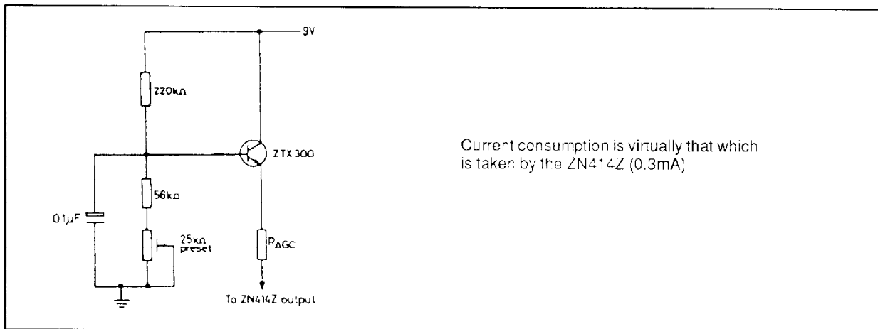
Fig. 9 Transistor Drive (ZN414Z and ZN415E)
