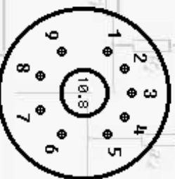
4 x 30° 3x40° 2.5φ PCφ: 24.5mm P9A
