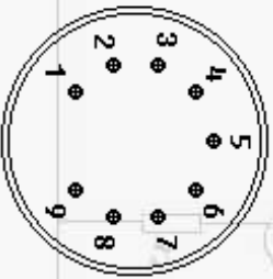
8 x 36° 1.02φ PCφ: 11.9mm B9A
