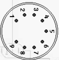
8 x 36° 1.27φ PCφ: 17.5mm B9D
